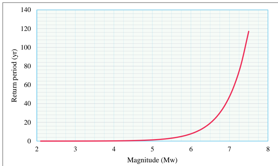
Fig. 7. Chart of different return periods and the maximum expected earthquake magnitudes
