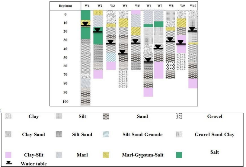
Figure 3. Well-logs of the study area
