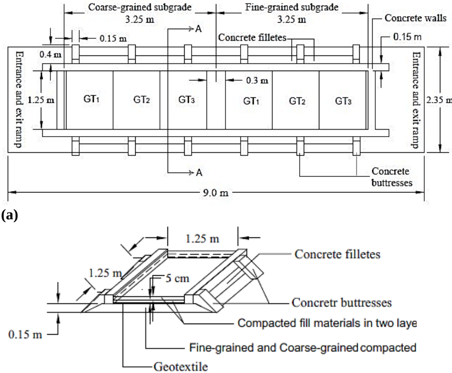
Figure 1. Schematic representation of the test setup (a) plan (b) section A-A [17], [27]
