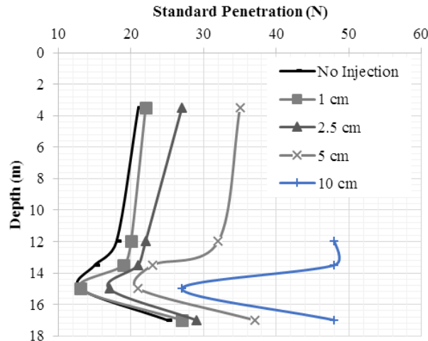
Figure7. Comparison of N_{SPT} changes with depth at micropiles distance of 3 meter.
