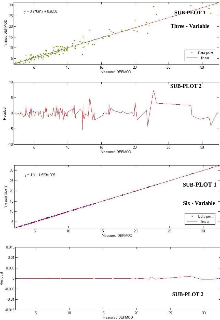
Figure 5. Analytically predictability estimation of the output structure of trained ANFISBSC comparing E_m (DEFMOD) measurements (Tab.3) versus modeled ones by ANFISBSC method (sub-plot 1) and residual values (sub-plot 2) for 3 and 6- variable simulations [8].
