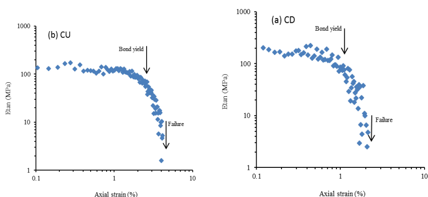
Figure 6. Bond yield and failure points for 0.5% fiber and 50% gravel content under 100 kPa confinement
