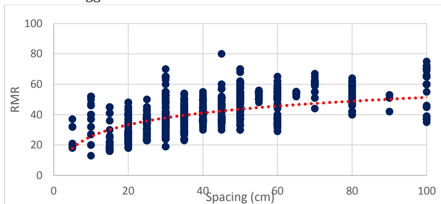
Fig. 6. The Relationship Between RMR Values and Joint Spacing
