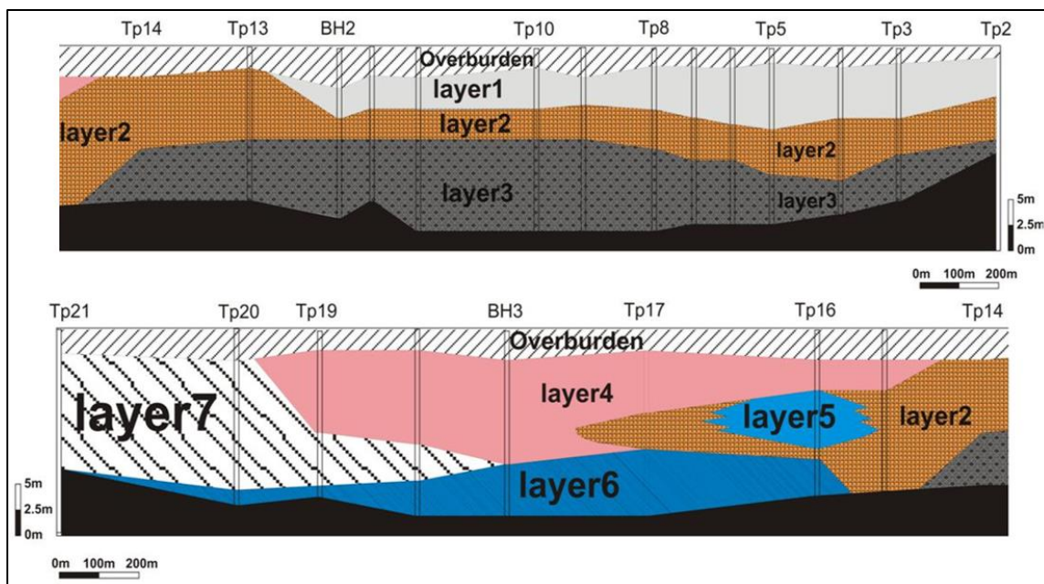
Fig. 5. Geotechnical profile of the study area
