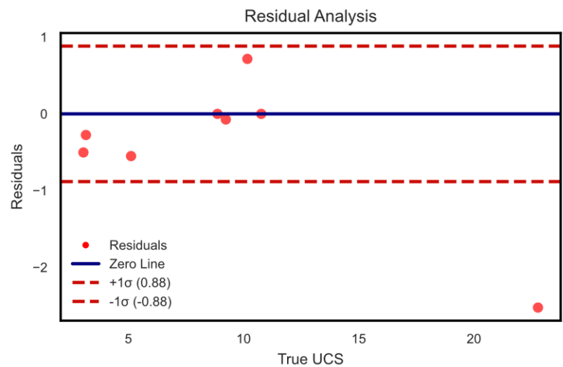
Fig. 9. Residual analysis to identify systematic biases
