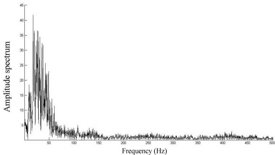
Fig. 9. The amplitude spectrum of thirtieth trace in Fig. 5 obtained from applying the first step of 2D median filter with 9 points window length on the indicated record in Fig. 3, and produced by MATLAB
