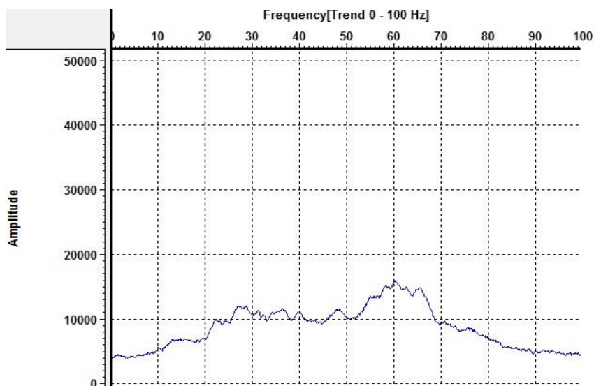
Fig. 21. The amplitude spectrum of the difference record displayed in Fig. 18 derived from VISTA software
