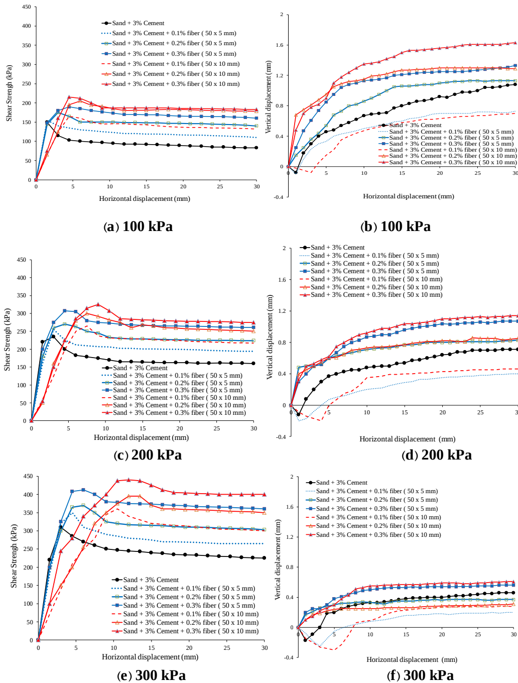
Fig. 4. (a) Shear stress-horizontal displacement curves of cemented sand and cemented sand reinforced with different percentages of 50 \times 5 mm and 50 \times 10 mm chips at 100 kPa; (b) vertical displacement-horizontal displacement curves for the same soils at surcharge pressure of 100 kPa; (c) shear stress-horizontal displacement curves of cemented sand and cemented sand reinforced with different percentages of 50 \times 5 mm and 50 \times 10 mm chips at 200 kPa; (d) vertical displacement-horizontal displacement curves of the same soil at surcharge pressure of 200 kPa; (e) shear stress-horizontal displacement curves of cemented sand and cemented sand reinforced with different percentages of 50 \times 5 mm and 50 \times 10 mm chips at surcharge pressure of 300 kPa; (f) vertical displacement-horizontal displacement curves for the same soils at surcharge pressure of 300 kPa.
