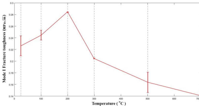
Figure 15. The fracture toughness of the concrete specimen at different temperatures
