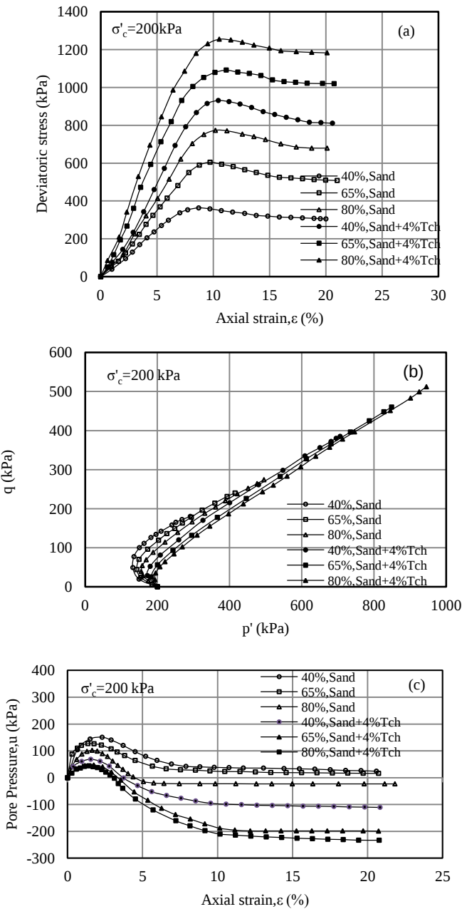
Figure 8. Effect of relative density on a) residual stress, b) effective stress path and c) pore water pressure
