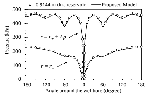
Figure 11. Comparison of pressure between three-cycle model and the proposed model
