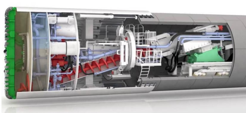
Figure 1. EPB Shield [1]
