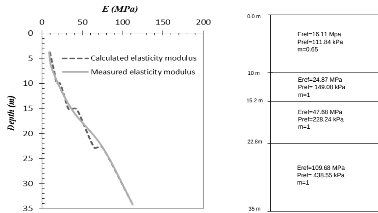
Figure 3. Fitting modulus of elasticity by Eq (1) in layered soil
