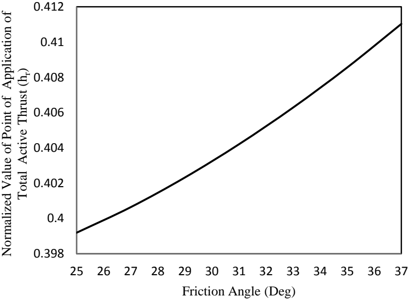
Fig.6. Variation of height ratio ( h_r ) with friction angle determined from present analysis for H = 10\text{ m}, \gamma = 18 \frac{kN}{m^3}
