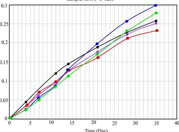
Expansion- Time diagram of aggregate Sample ASTM- C 1260
