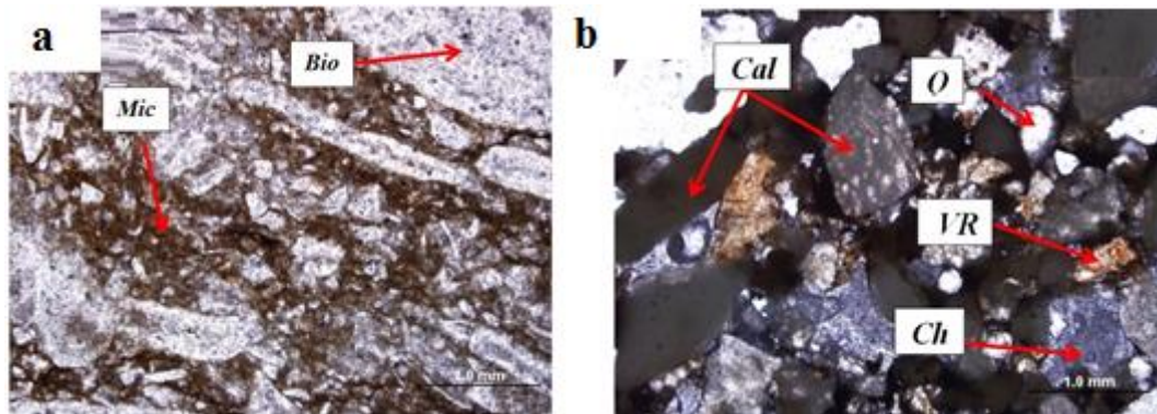
Figure 3. Microscopic image of microscopic thin sections a) Limestone, and b) Sandstone Micrite (Mic), fossil (Bio), chert (Ch), limestone (Cal), and igneous (VR fragments), quartz (Q)
