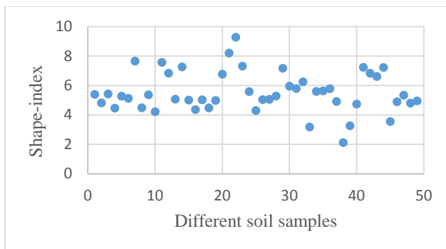
Figure 5. Shape index of the collected soil samples.
