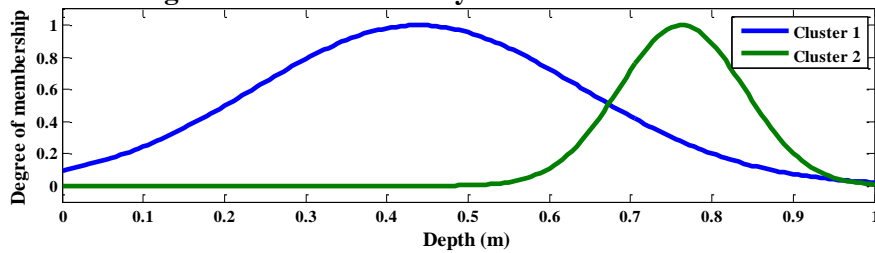
Figure 5. MFs obtained by ANFIS-SCM model
