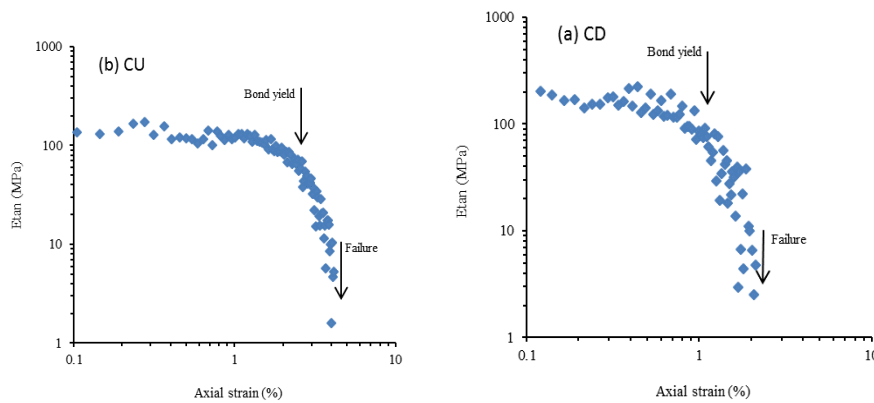
Figure 6. Bond yield and failure points for 0.5% fiber and 50% gravel content under 100 kPa confinement a) Consolidated-Drained b) Consolidated Undrained
