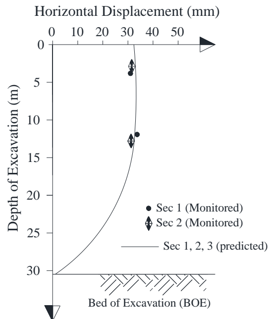
Figure 8. Comparison between results of FE model and monitoring data Numerical results and discussion
