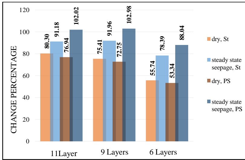
Figure 12. Horizontal displacement variations in inclined layered models
